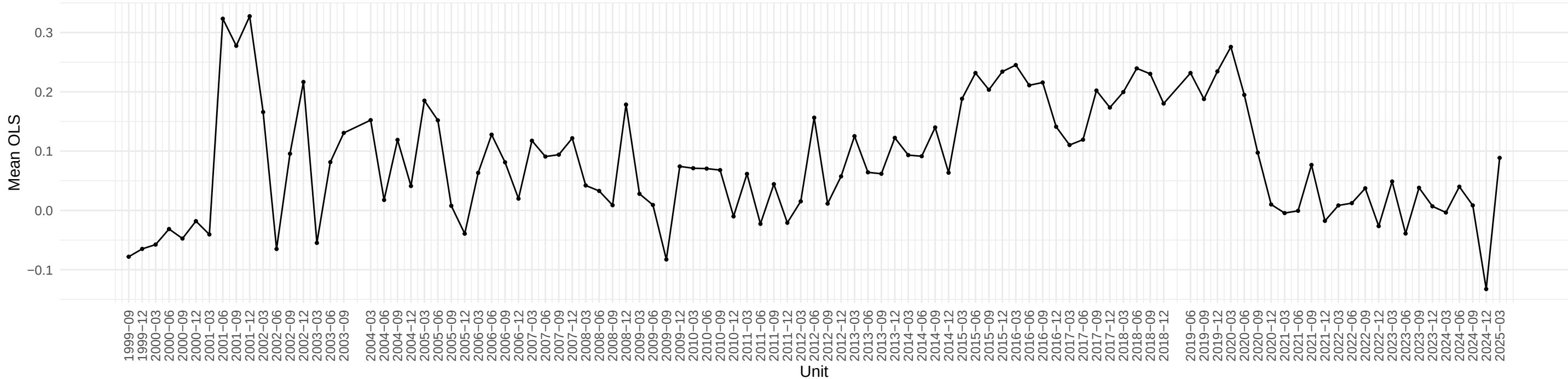
Evolution of ISRATIOx OLS coefficient across time
