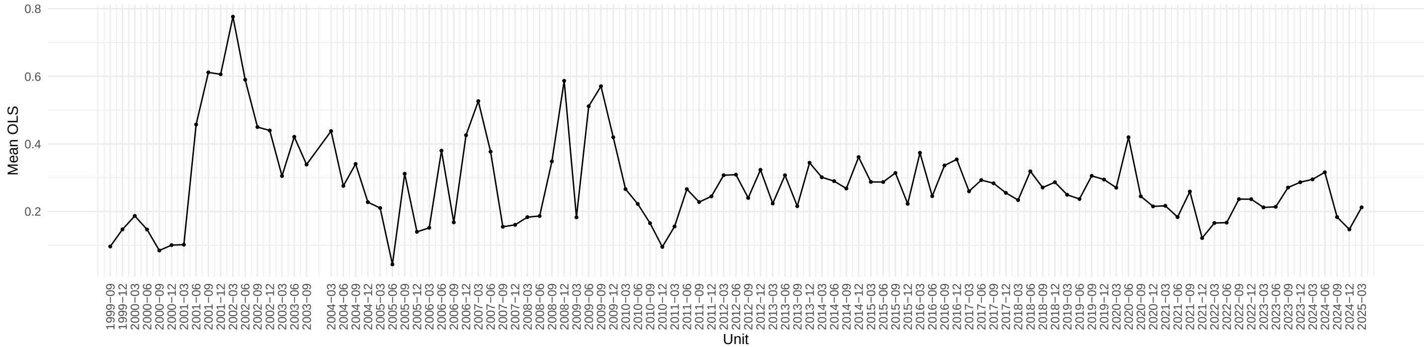
Evolution of PERMITMW OLS coefficient across time
