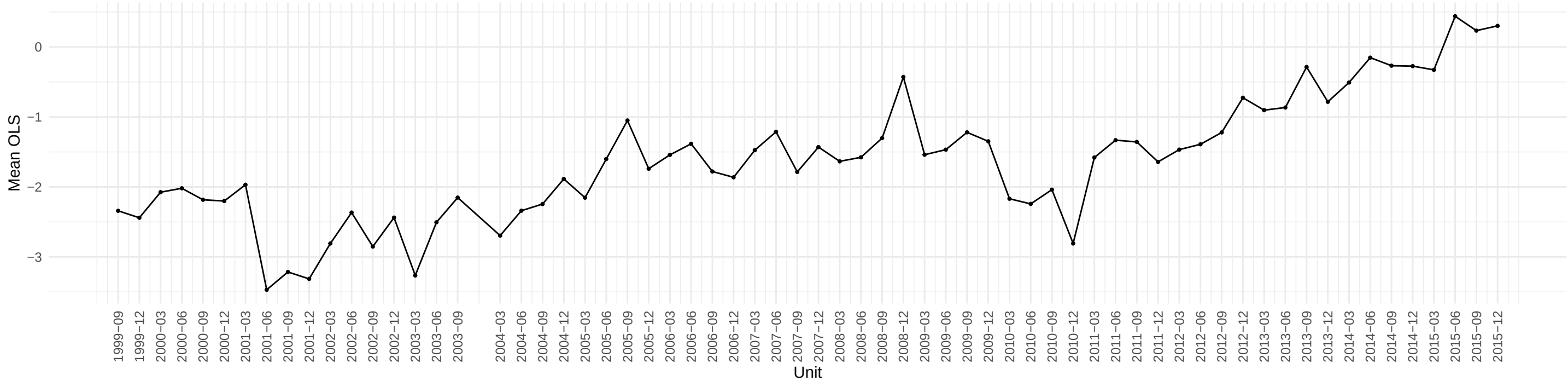
Evolution of PPICRM OLS coefficient across time
