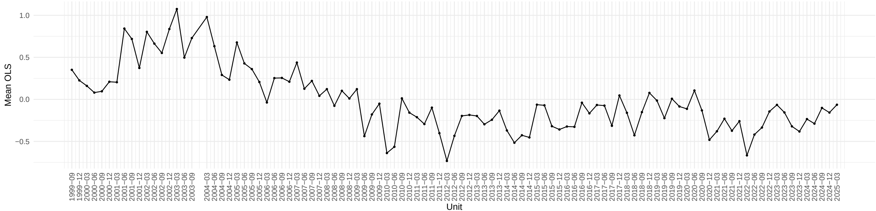
Evolution of TB6SMFFM OLS coefficient across time
