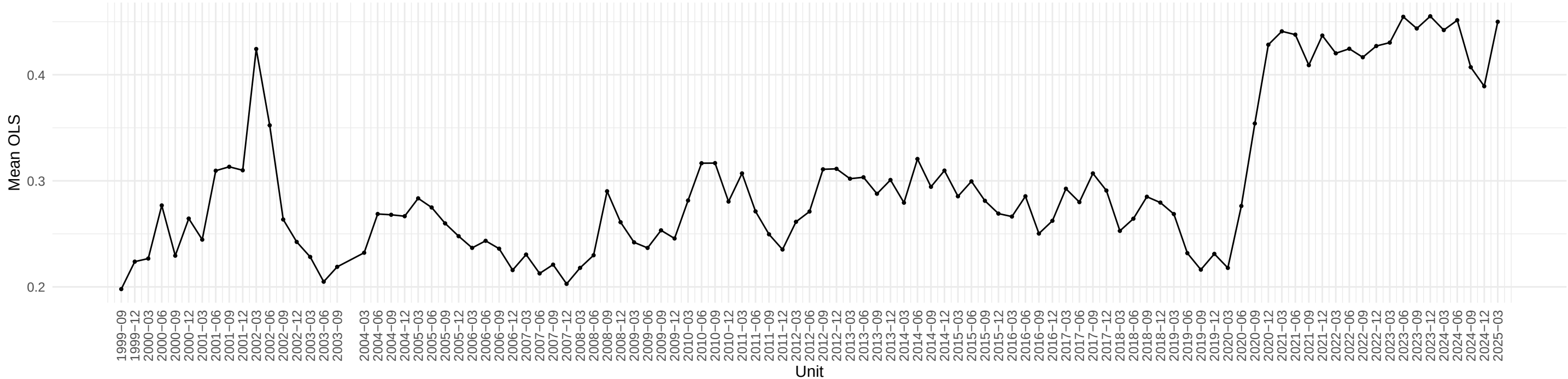
Evolution of UEMP5TO14 OLS coefficient across time
