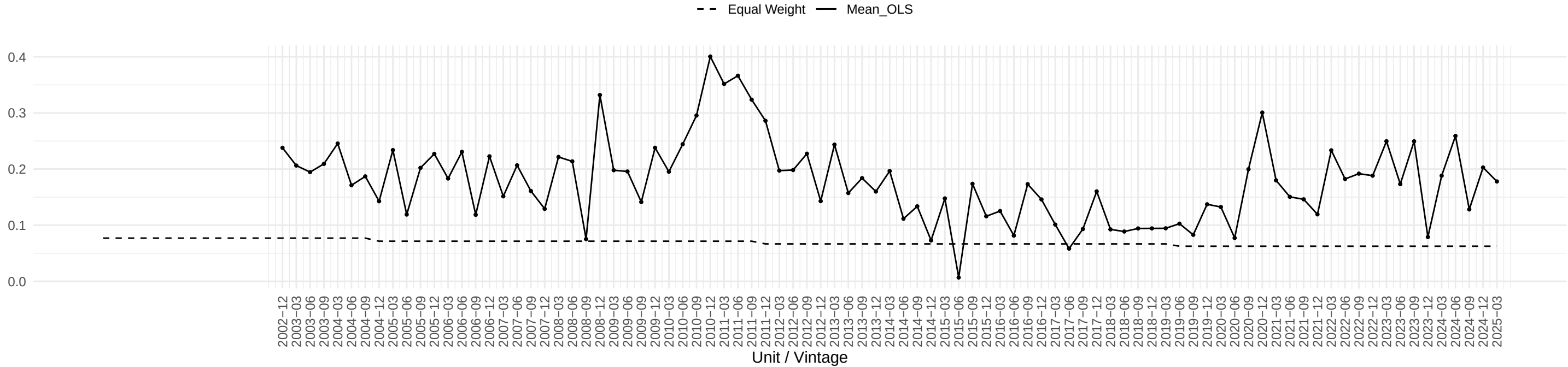
Evolution of IPNCONGD OLS coefficient across time
