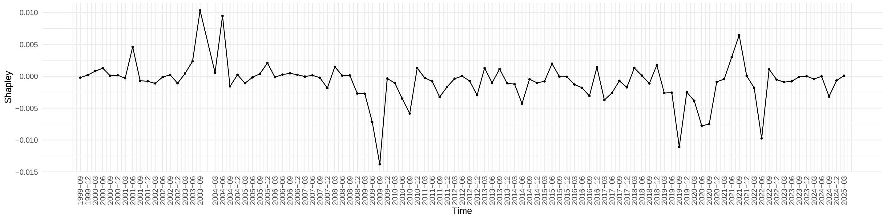
Evolution of Shapley Value of BAA across time
