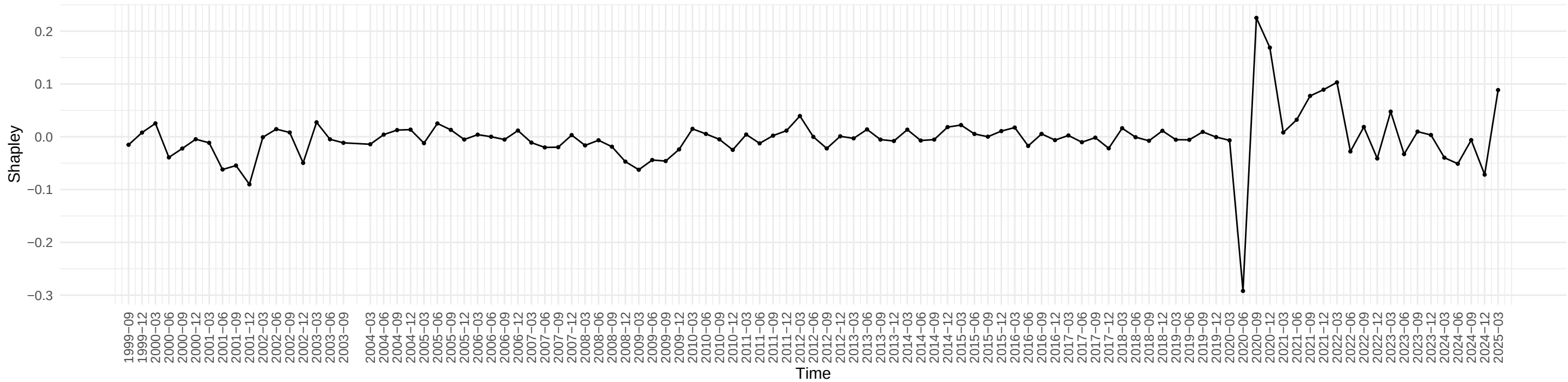
Evolution of Shapley Value of CE16OV across time
