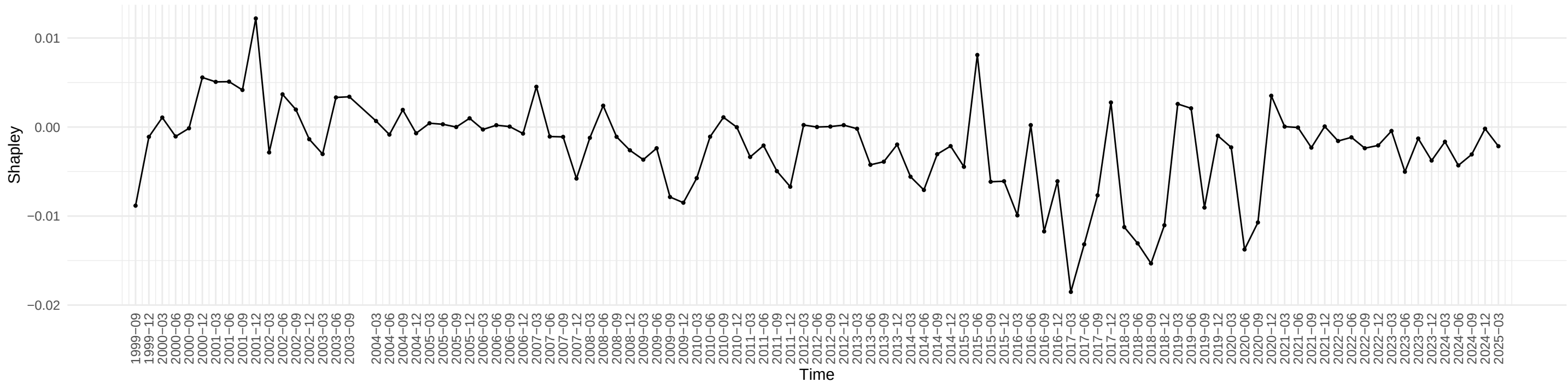
Evolution of Shapley Value of CES0600000008 across time
