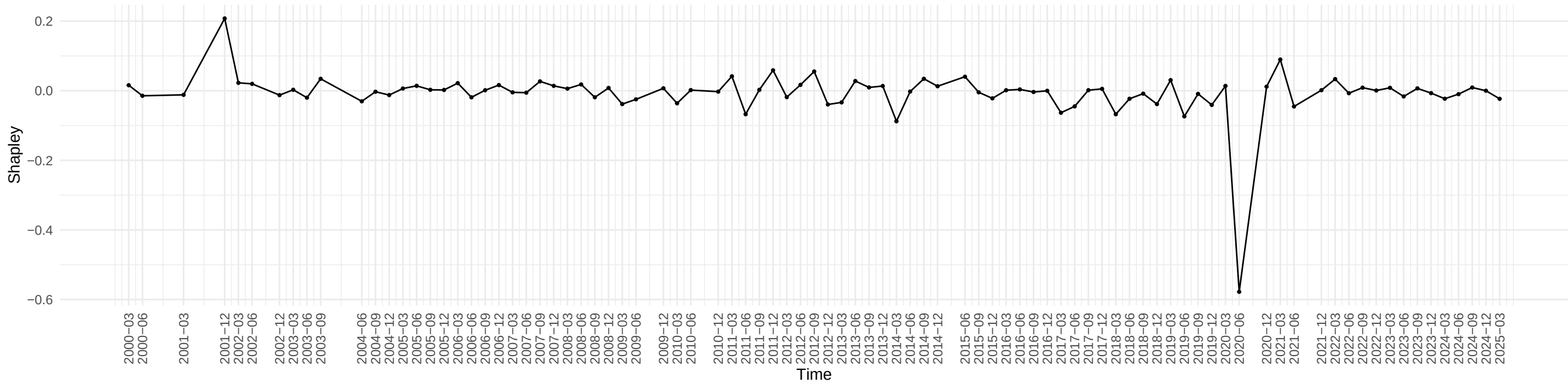
Evolution of Shapley Value of CMRMTSPLx across time
