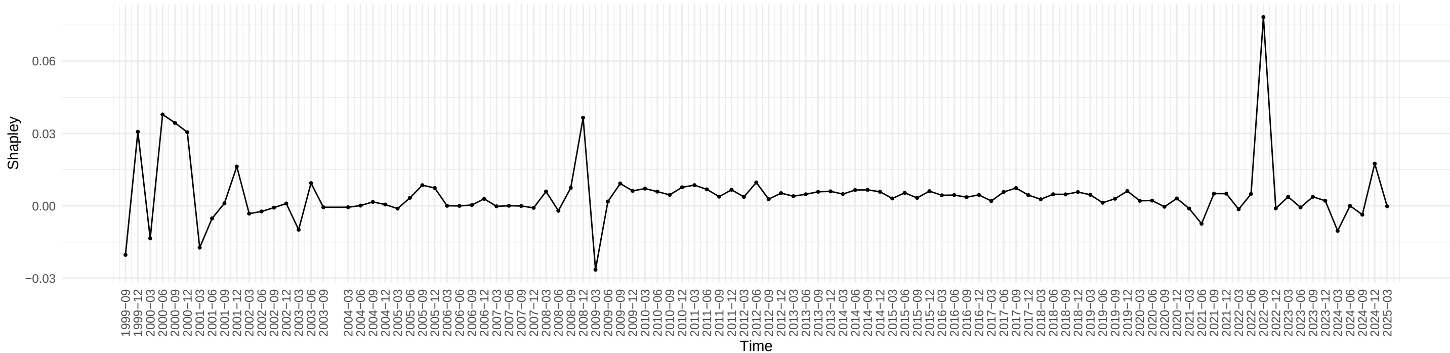
Evolution of Shapley Value of CUSR0000SAC across time
