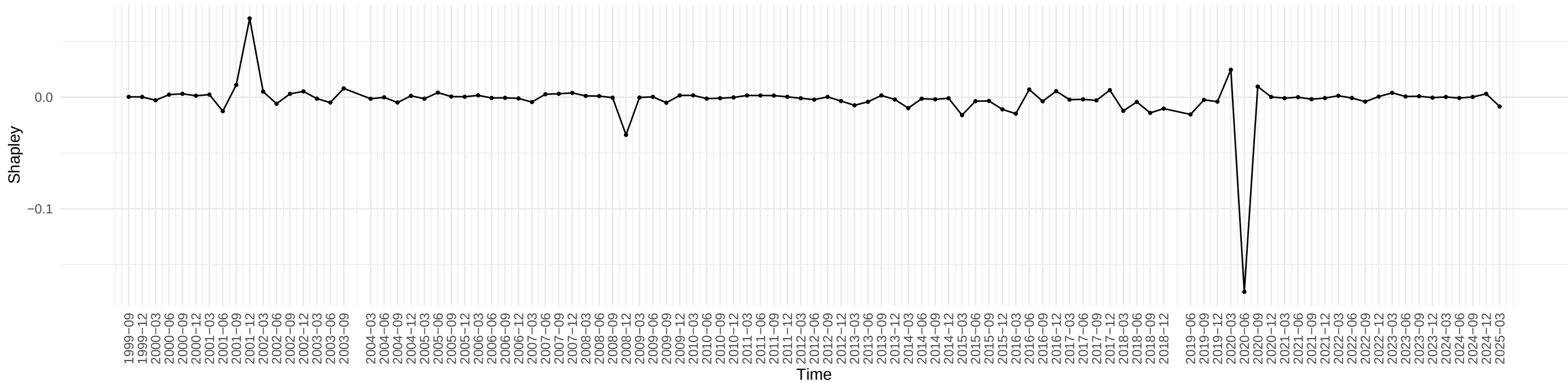
Evolution of Shapley Value of ISRATIOx across time
