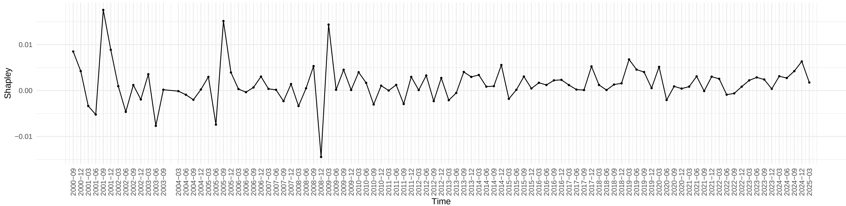
Evolution of Shapley Value of PCEPI across time
