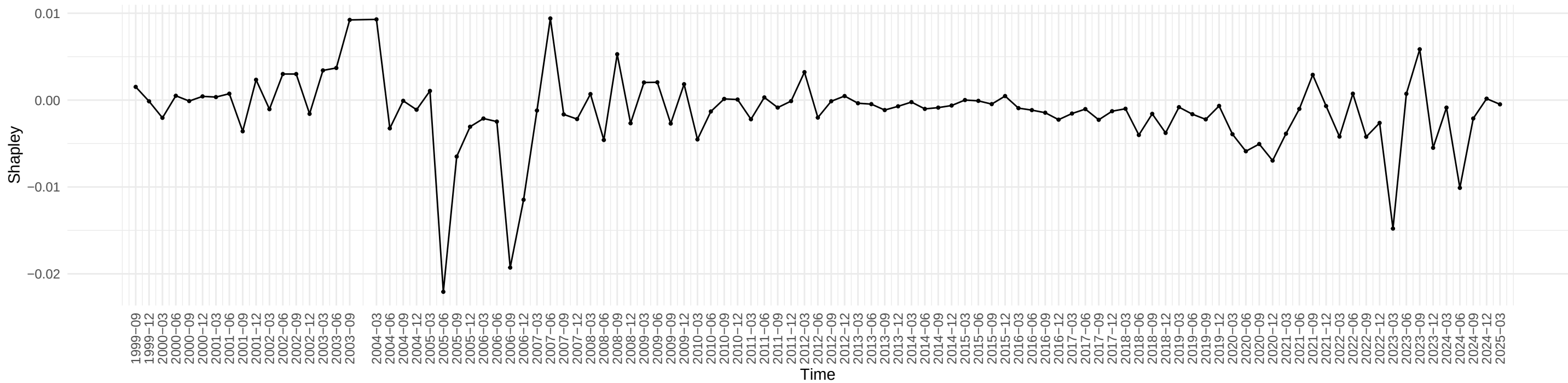
Evolution of Shapley Value of REALLN across time
