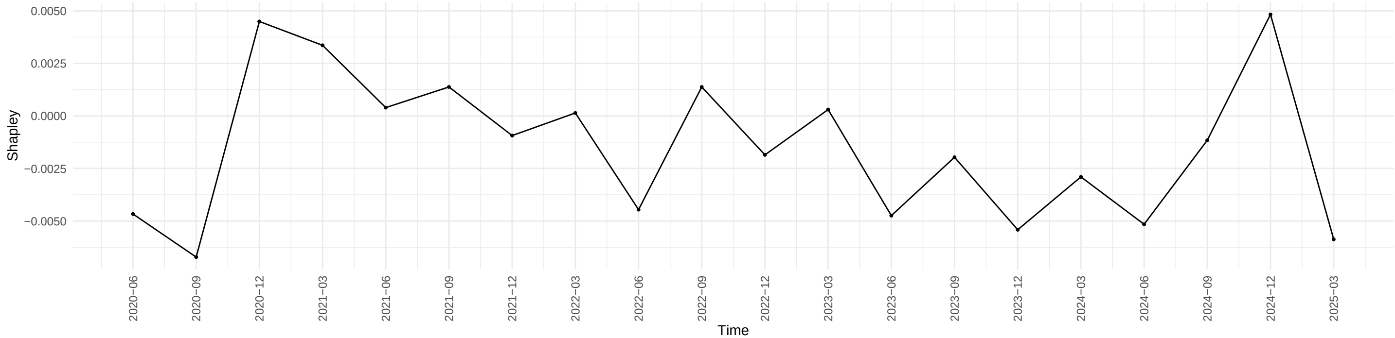
Evolution of Shapley Value of TWEXAFEGSMTHx across time
