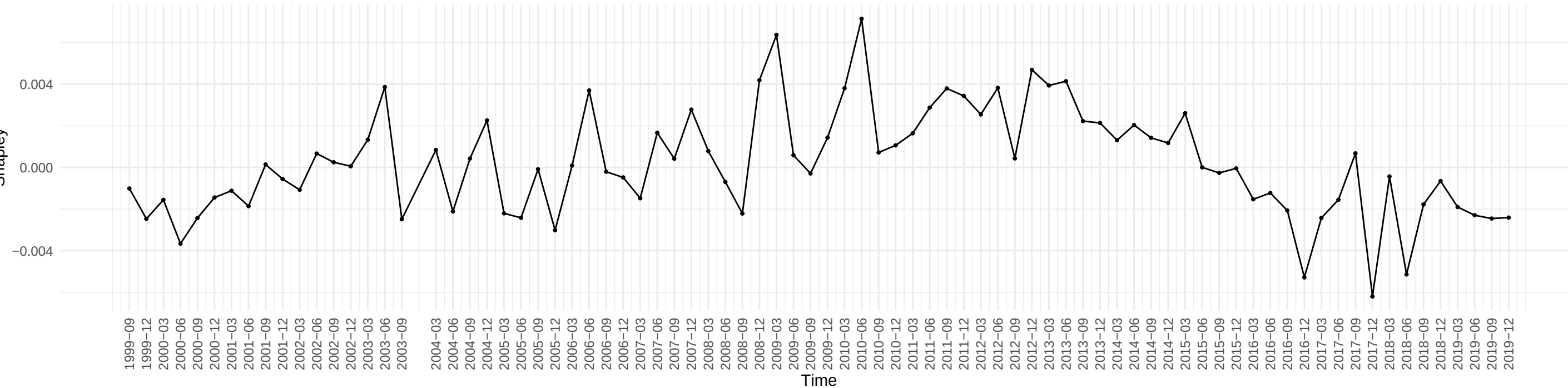
Evolution of Shapley Value of TWEXMMTH across time
