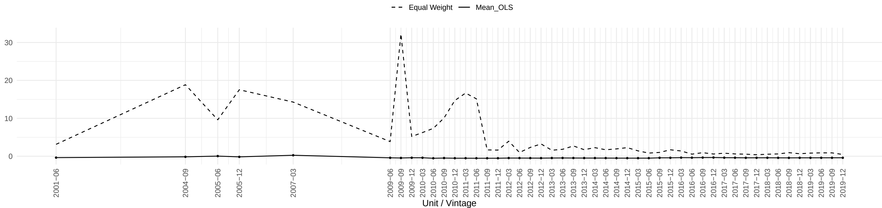
Evolution of AMBSL OLS coefficient across time
