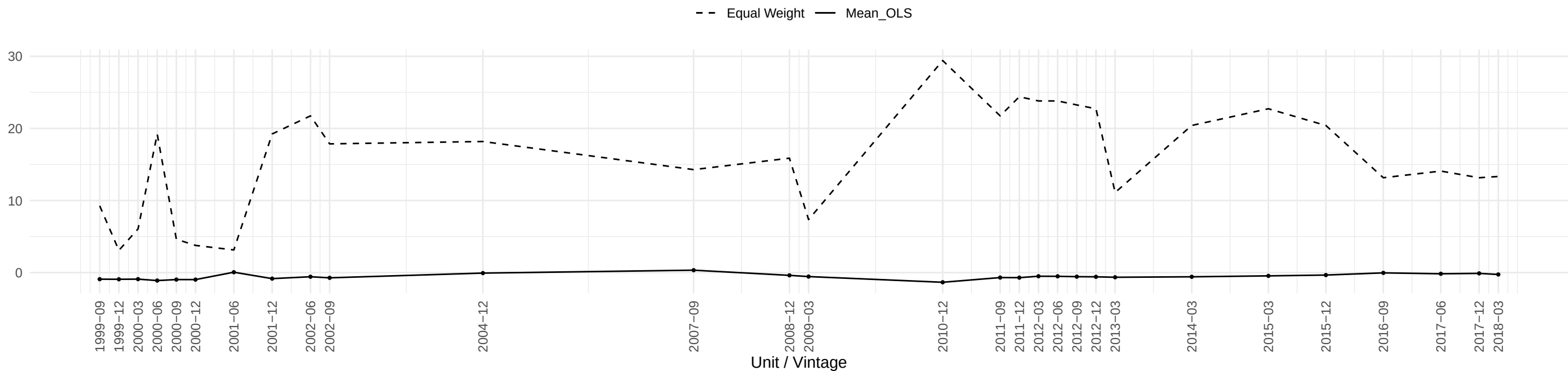
Evolution of CPITRNSL OLS coefficient across time
