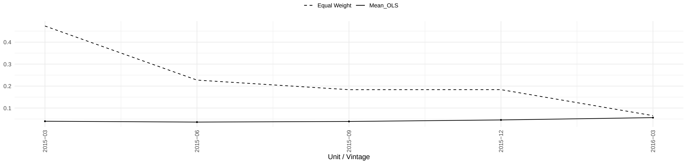
Evolution of NAPMPI OLS coefficient across time
