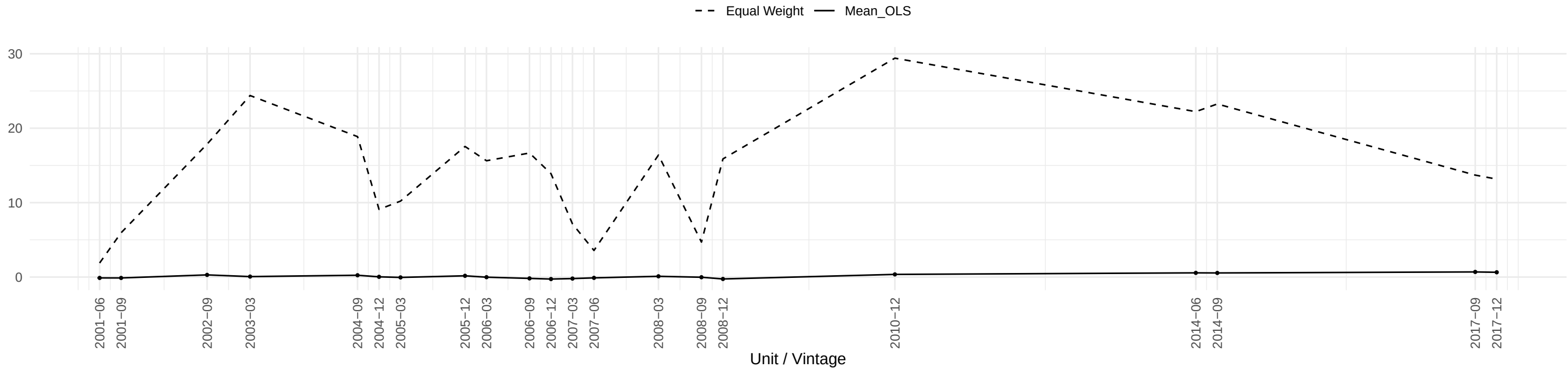
Evolution of UMCSENTx OLS coefficient across time
