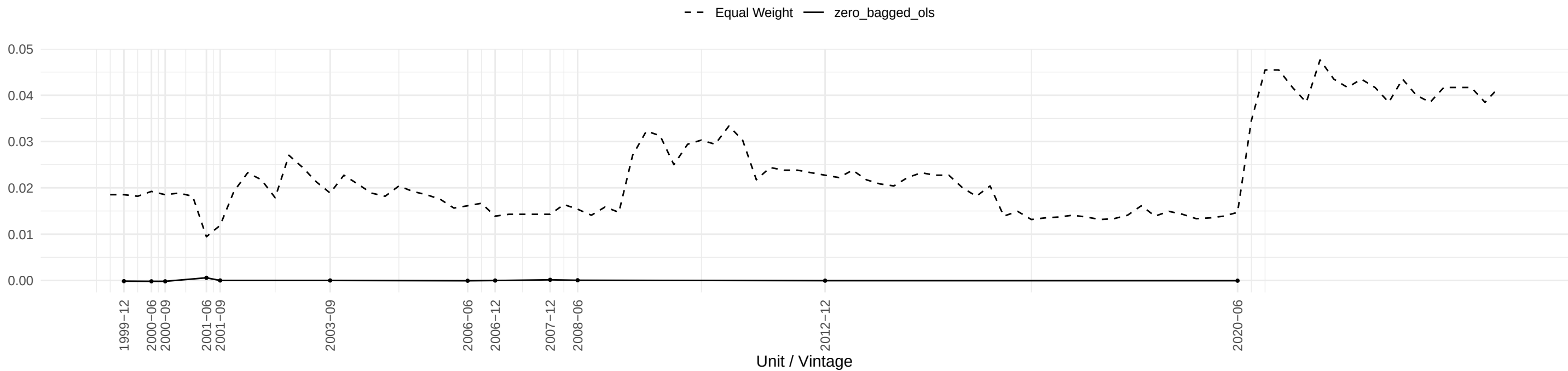
Evolution of AAA OLS coefficient across time
