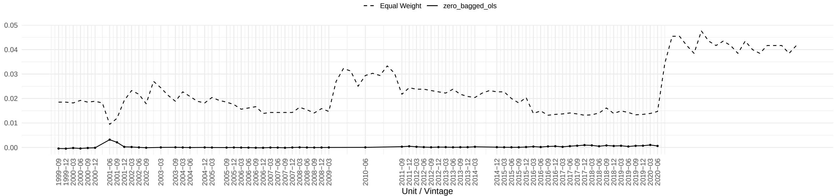
Evolution of AMDMNOx OLS coefficient across time
