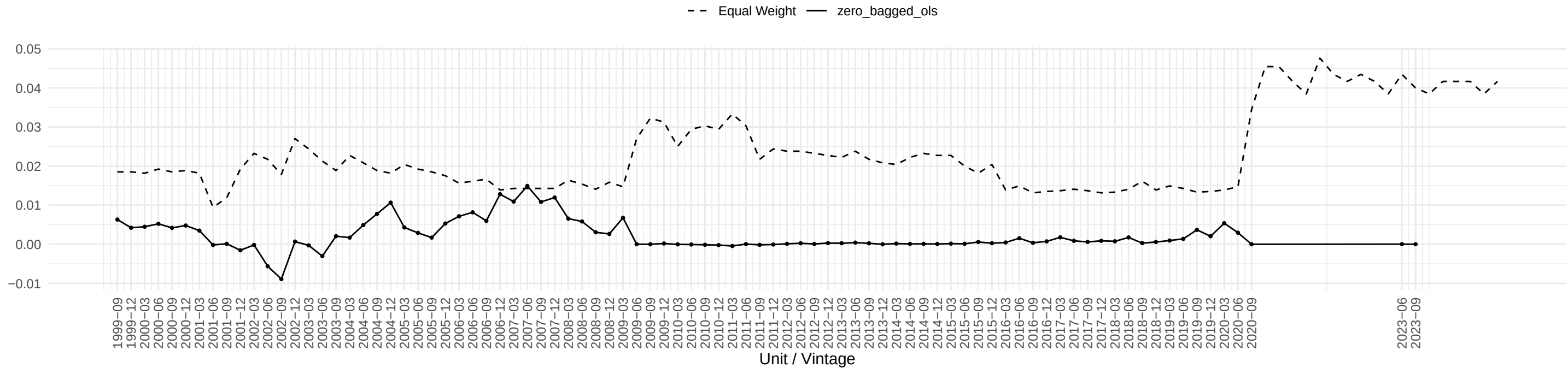
Evolution of AWHMAN OLS coefficient across time
