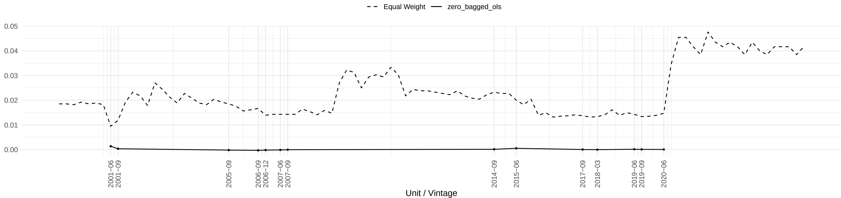
Evolution of BAA OLS coefficient across time
