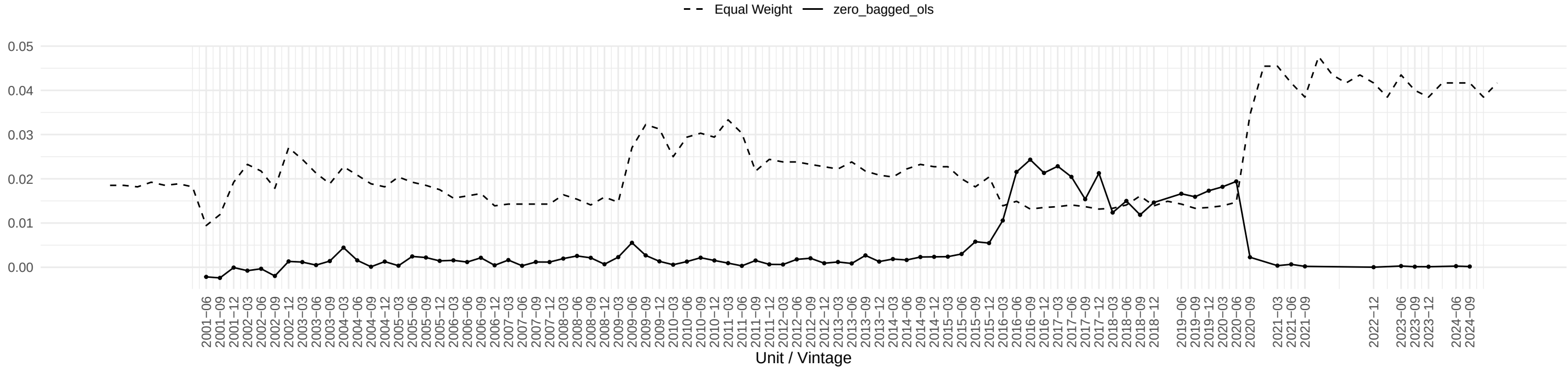
Evolution of BUSINVx OLS coefficient across time
