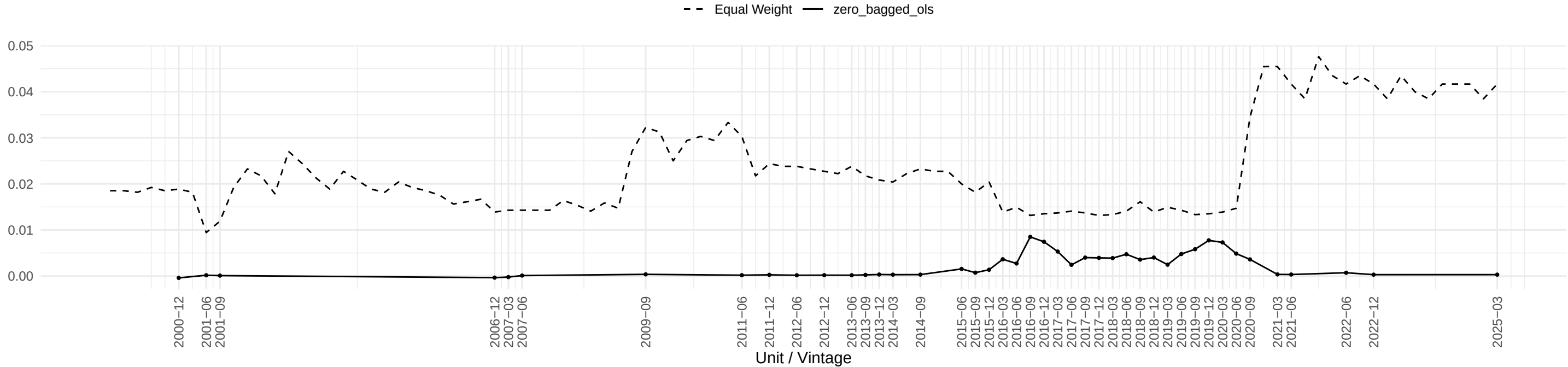
Evolution of CES1021000001 OLS coefficient across time
