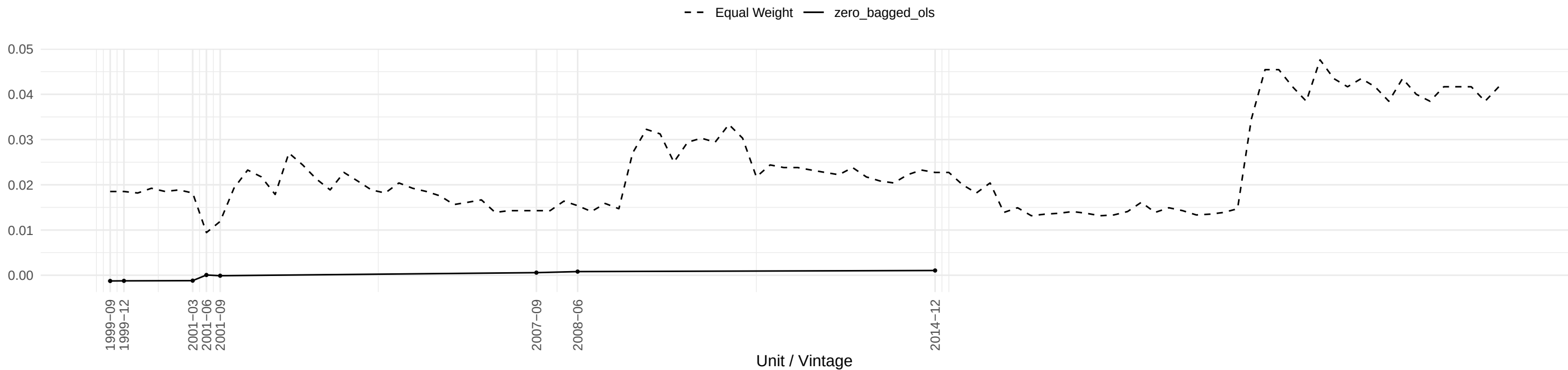
Evolution of CPIAPPSL OLS coefficient across time
