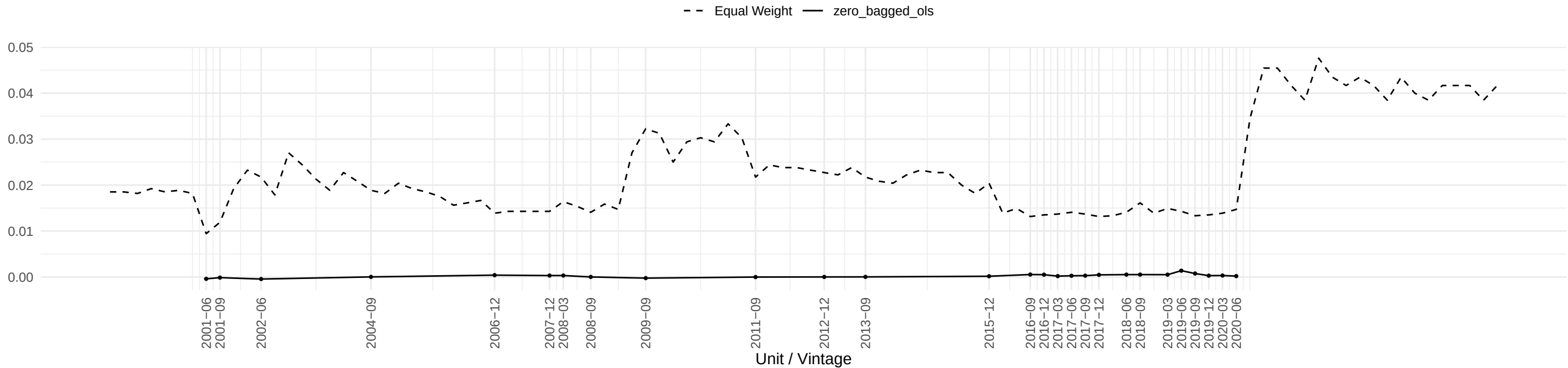
Evolution of CPIAUCSL OLS coefficient across time
