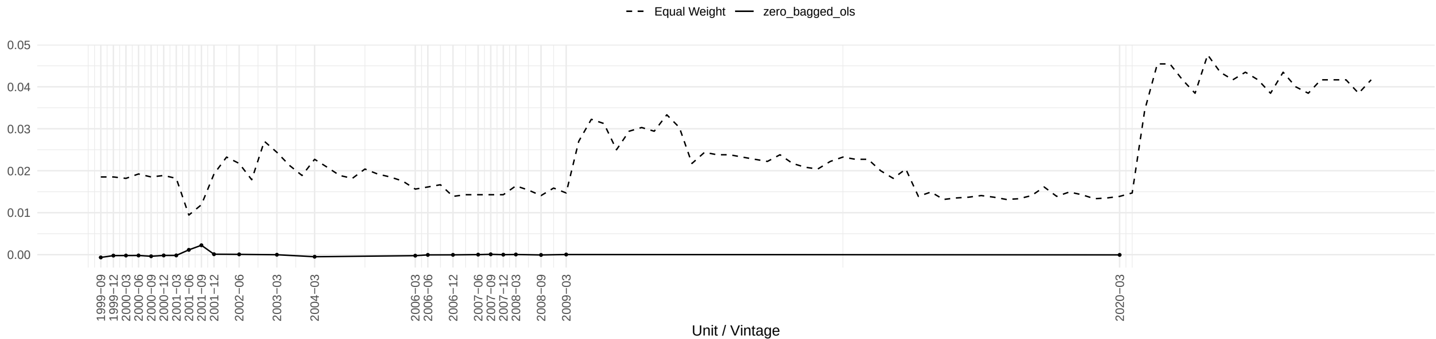
Evolution of GS5 OLS coefficient across time
