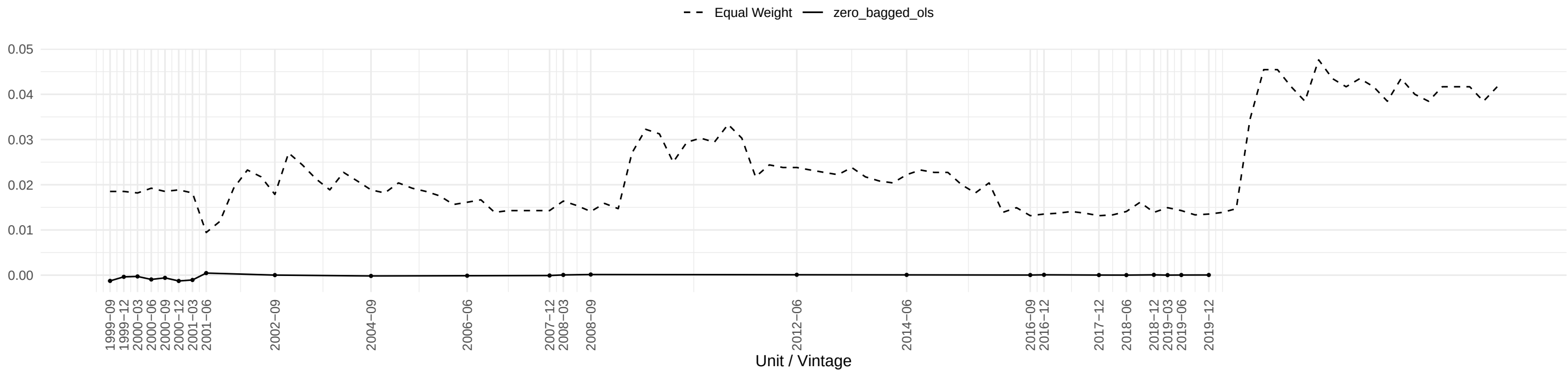
Evolution of HOUST OLS coefficient across time
