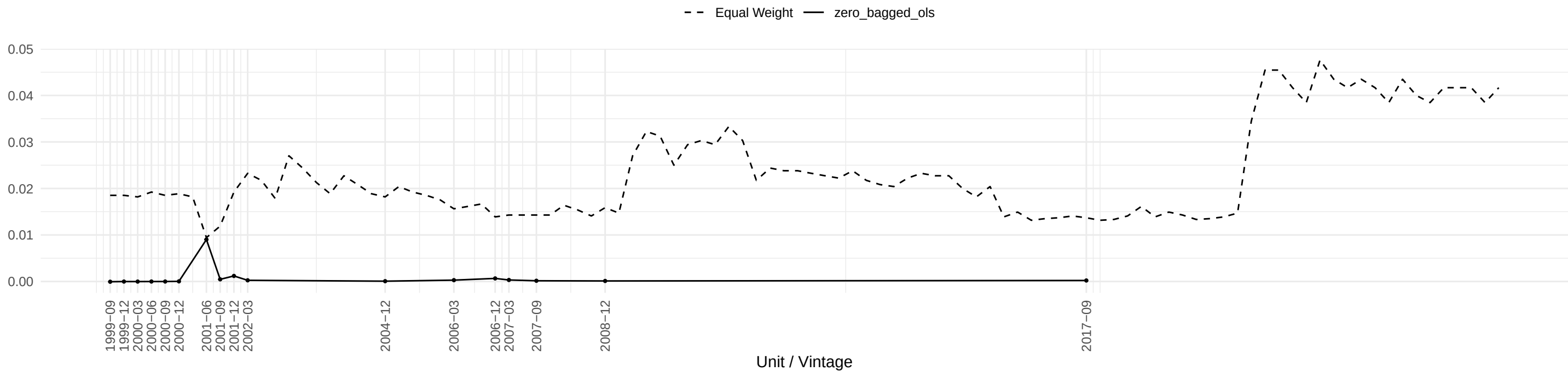
Evolution of MZMSL OLS coefficient across time
