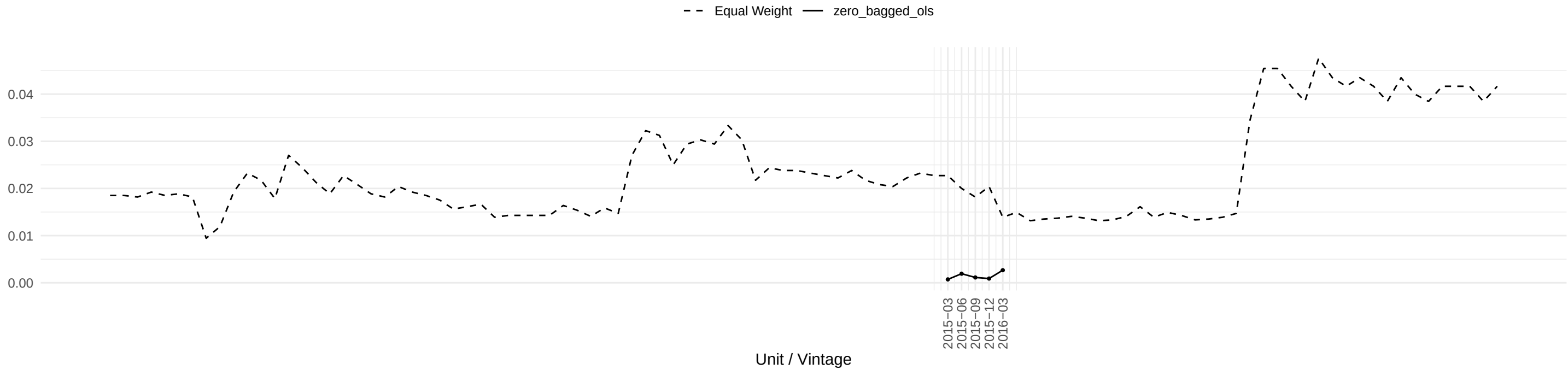
Evolution of NAPMNOI OLS coefficient across time
