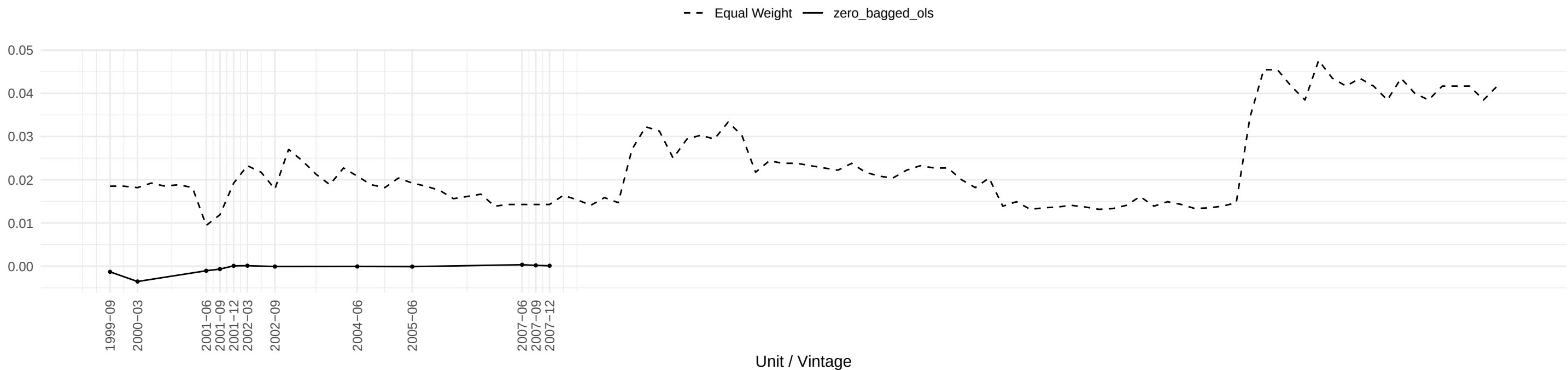
Evolution of NONBORRES OLS coefficient across time
