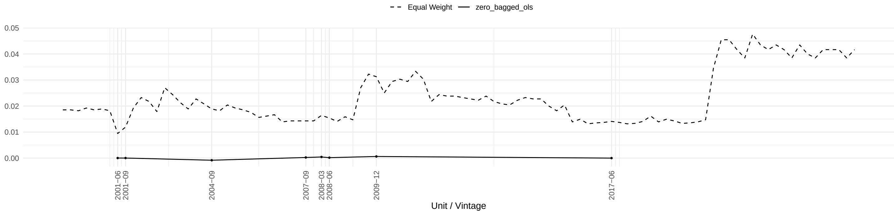
Evolution of NONREVSL OLS coefficient across time
