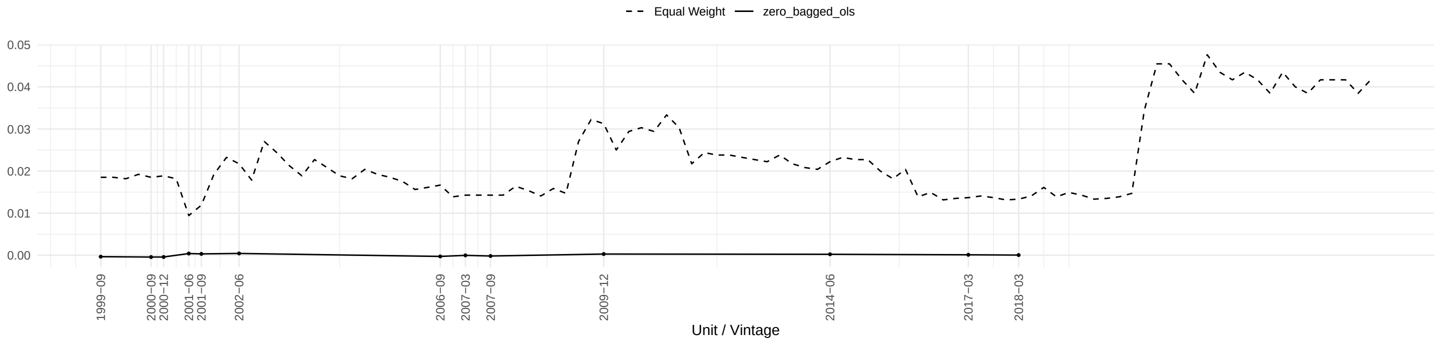
Evolution of PERMITS OLS coefficient across time
