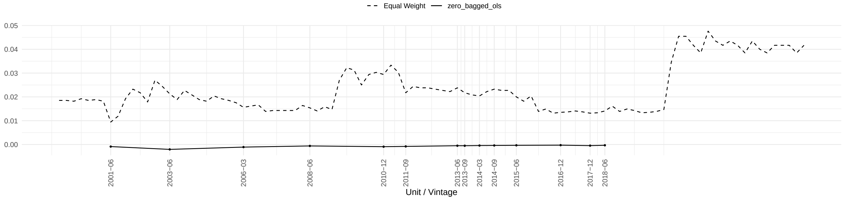
Evolution of PPICMM OLS coefficient across time
