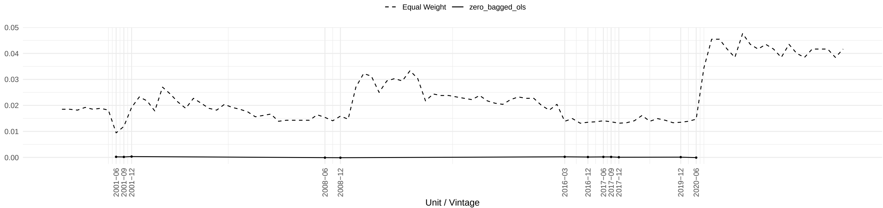
Evolution of RETAILx OLS coefficient across time
