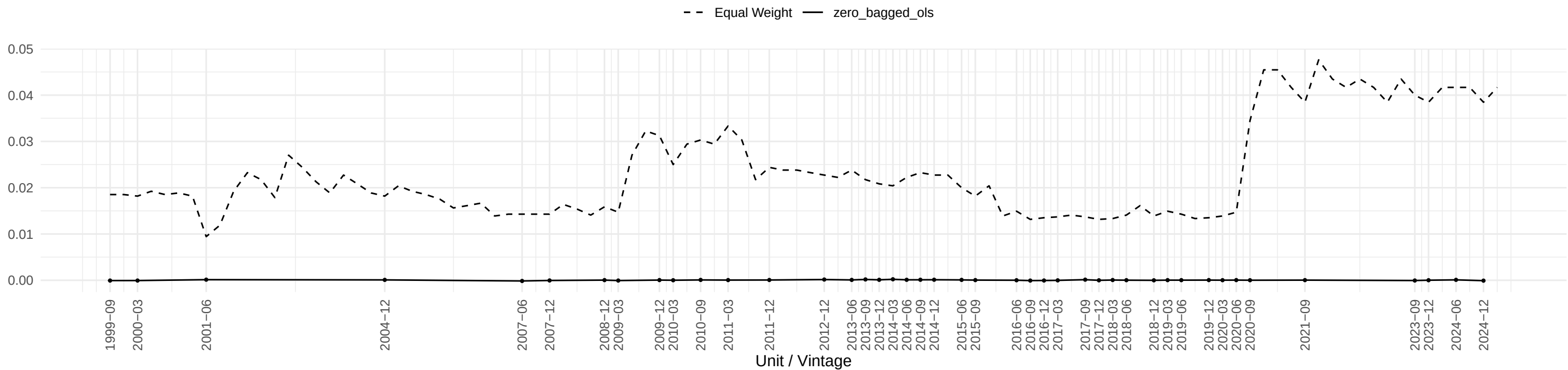
Evolution of USFIRE OLS coefficient across time
