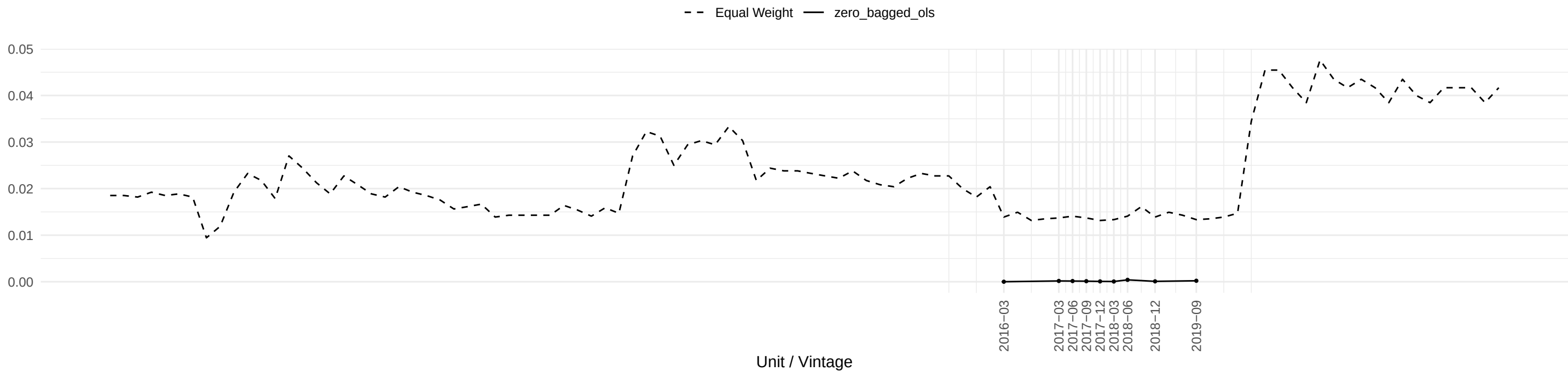
Evolution of WPSFD49502 OLS coefficient across time
