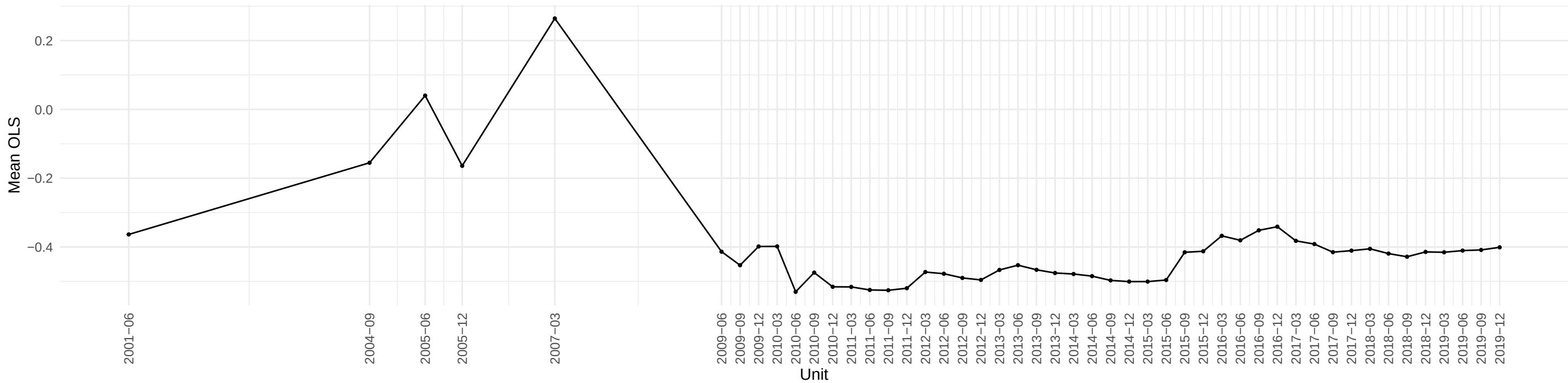
Evolution of AMBSL OLS coefficient across time
