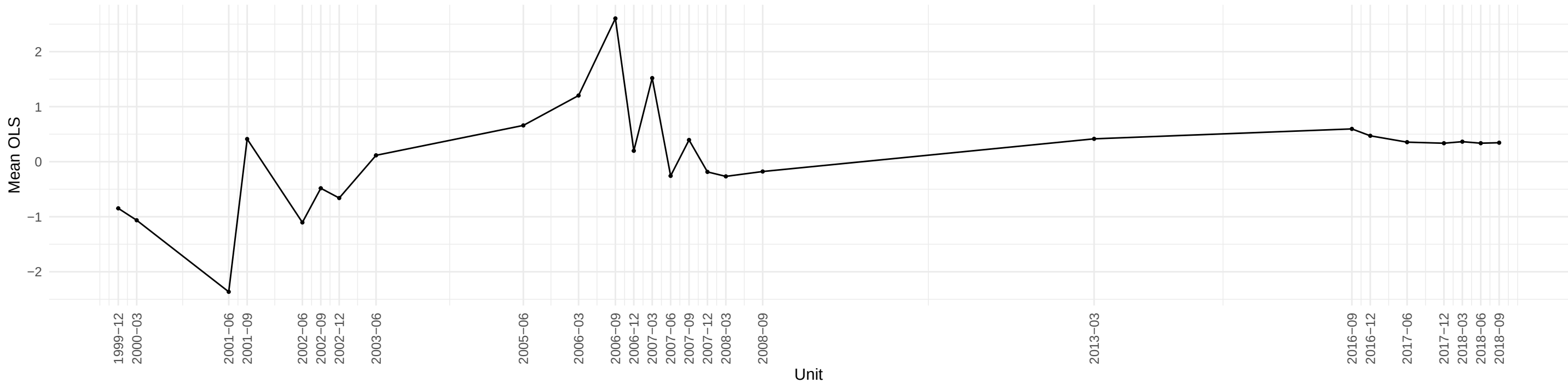
Evolution of BAAFFM OLS coefficient across time
