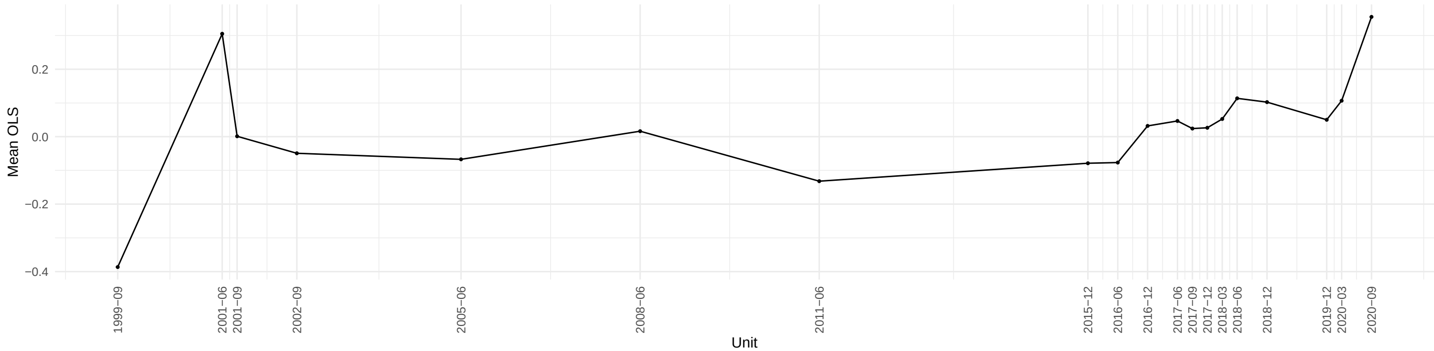
Evolution of BUSLOANS OLS coefficient across time
