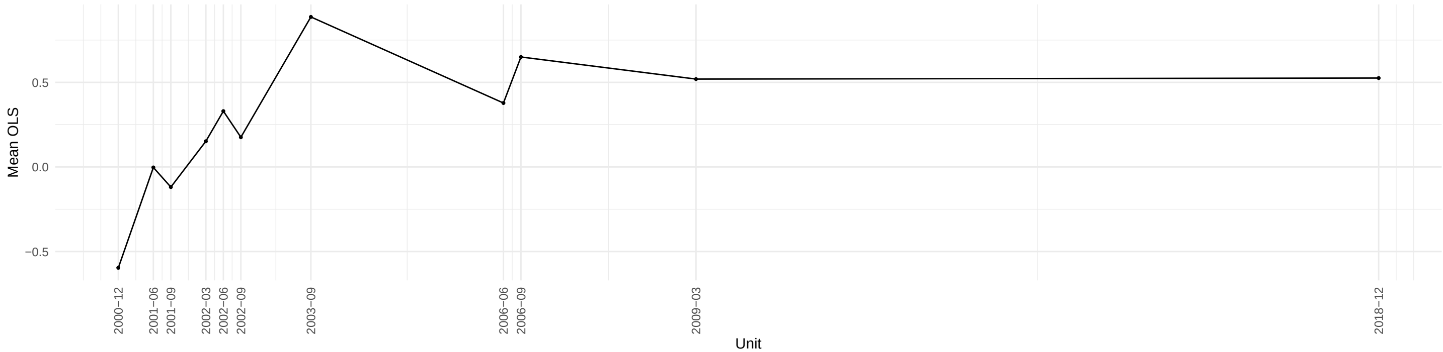
Evolution of CLF16OV OLS coefficient across time
