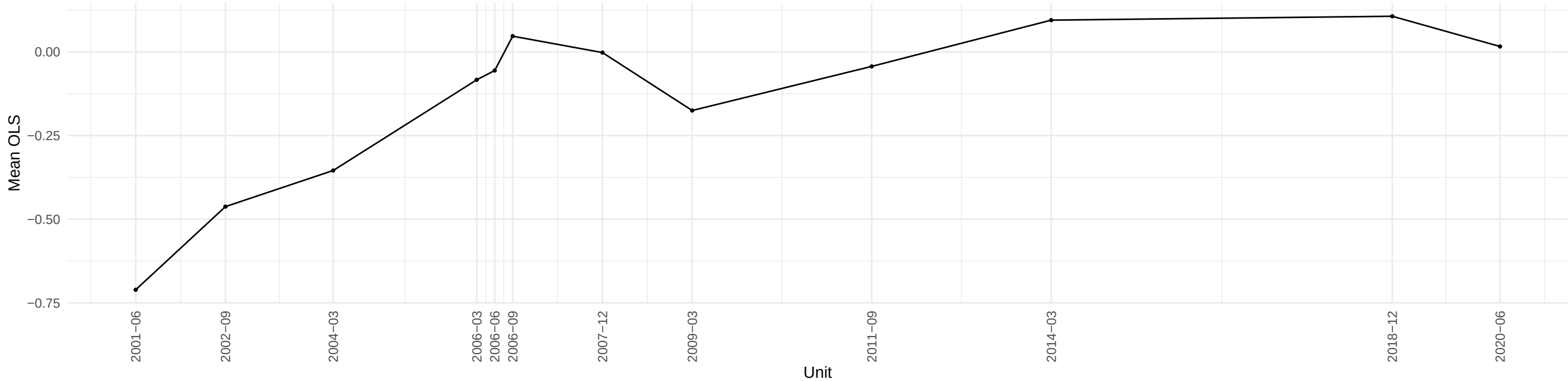
Evolution of CONSPI OLS coefficient across time
