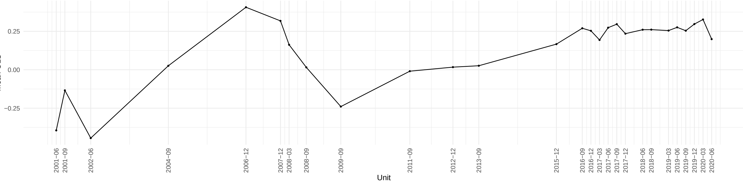
Evolution of CPIAUCSL OLS coefficient across time
