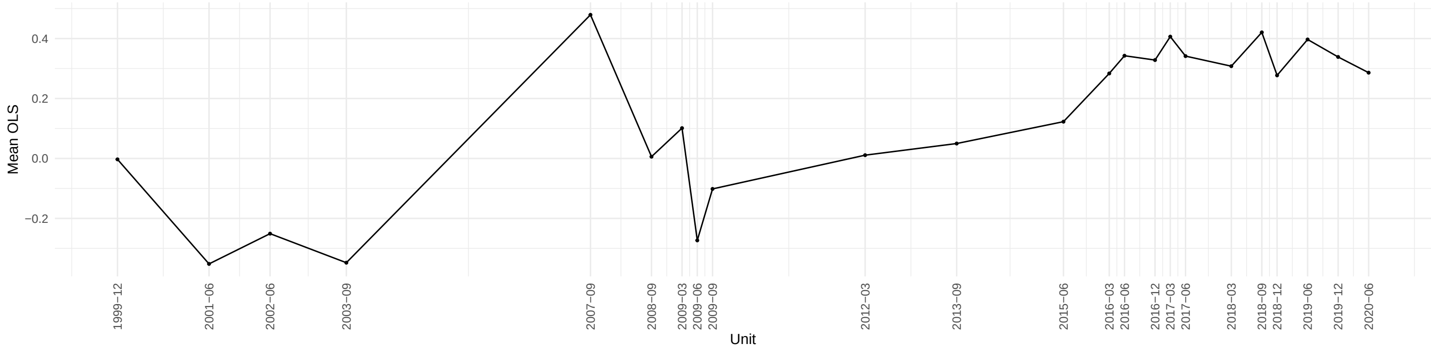
Evolution of CUSR0000SA0L5 OLS coefficient across time
