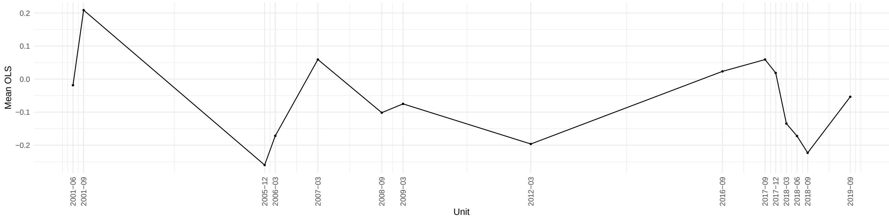
Evolution of EXSZUSx OLS coefficient across time
