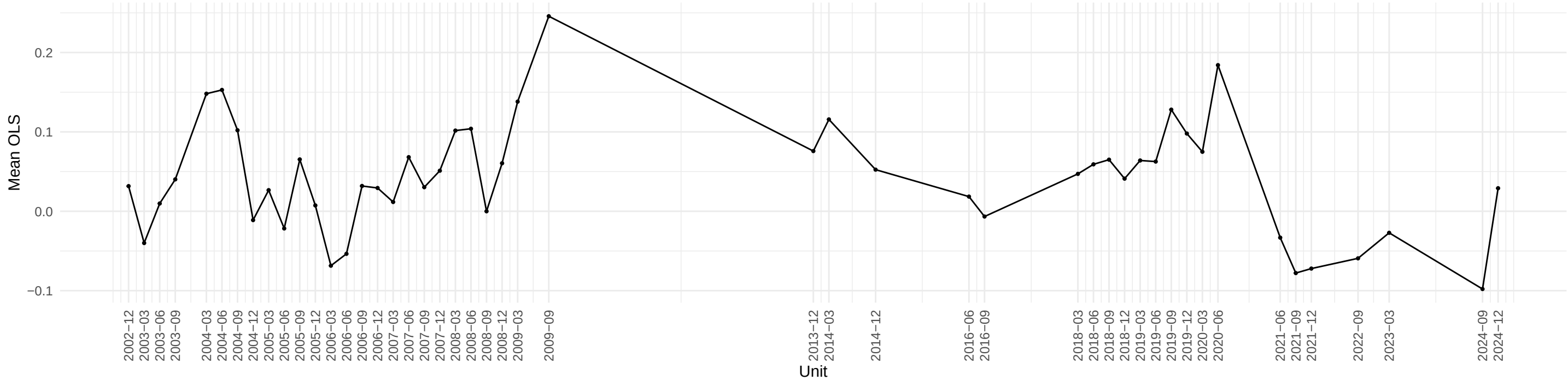
Evolution of IPNMAT OLS coefficient across time
