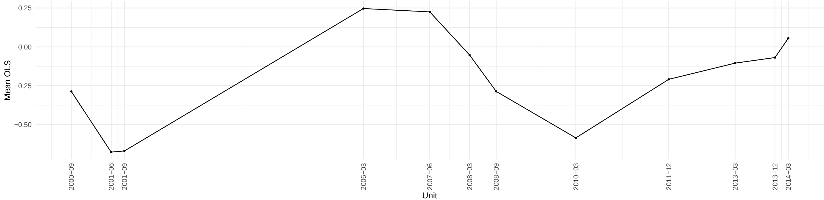
Evolution of PPIFGS OLS coefficient across time
