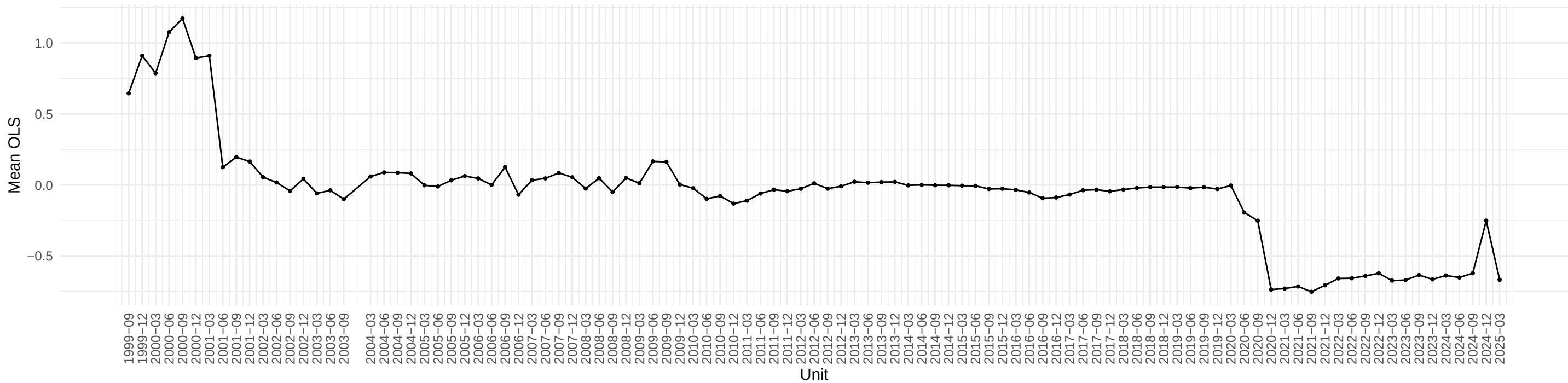
Evolution of SRVPRD OLS coefficient across time
